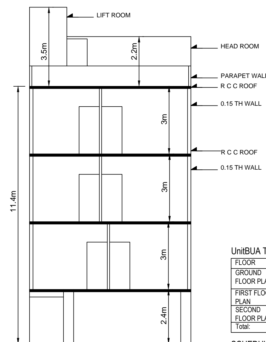
SECTION @ X-X
